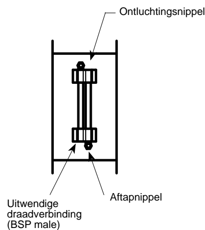
Type NJOG . 00
